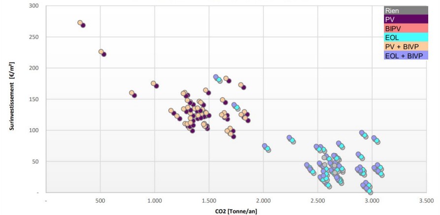
COMPARAISON Concepts globaux Surinvestissement [€/m 2 ] / CO2 [Tonne/an]
